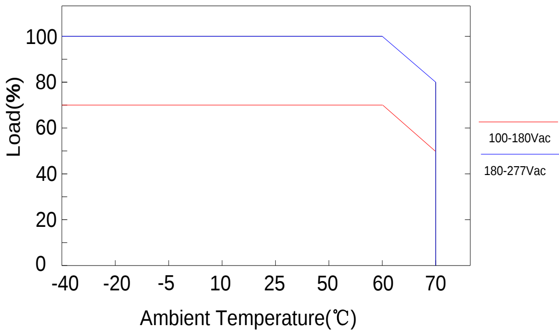
Derating Curve
