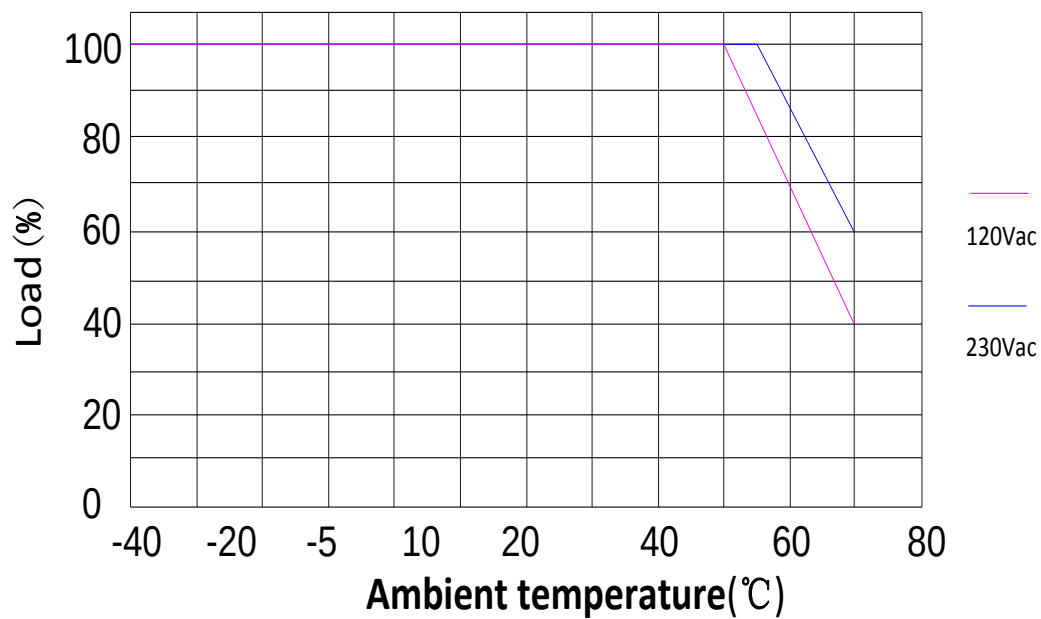
Derating curve
