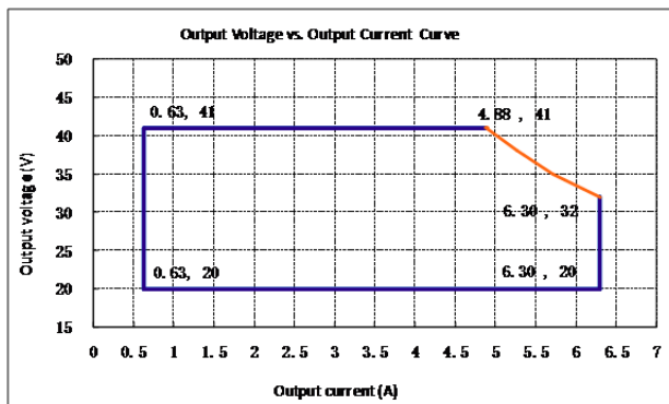
LDP-200X120 -A
