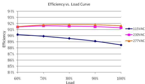
LDP-200X120-A(U=72V)
