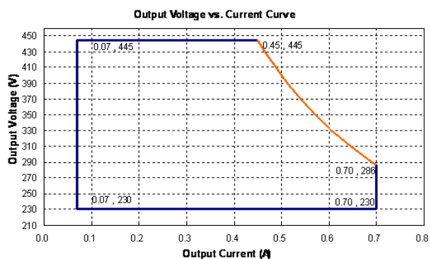
LDP-200X445
