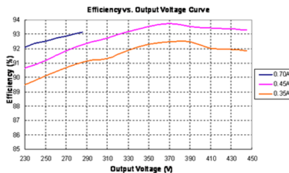
LDP-200X445(Vin=230Vac)
