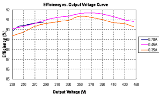
LDP-200X445(Vin=115Vac)
