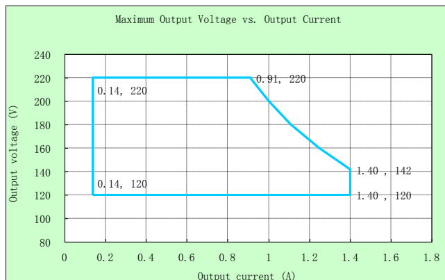
LDP-200X445
