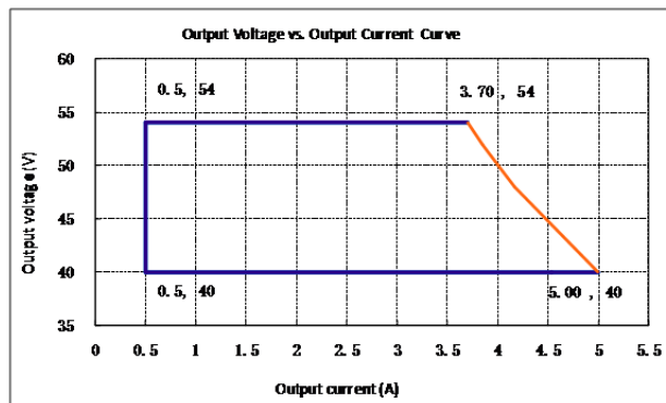
LDP-200X120 -B
