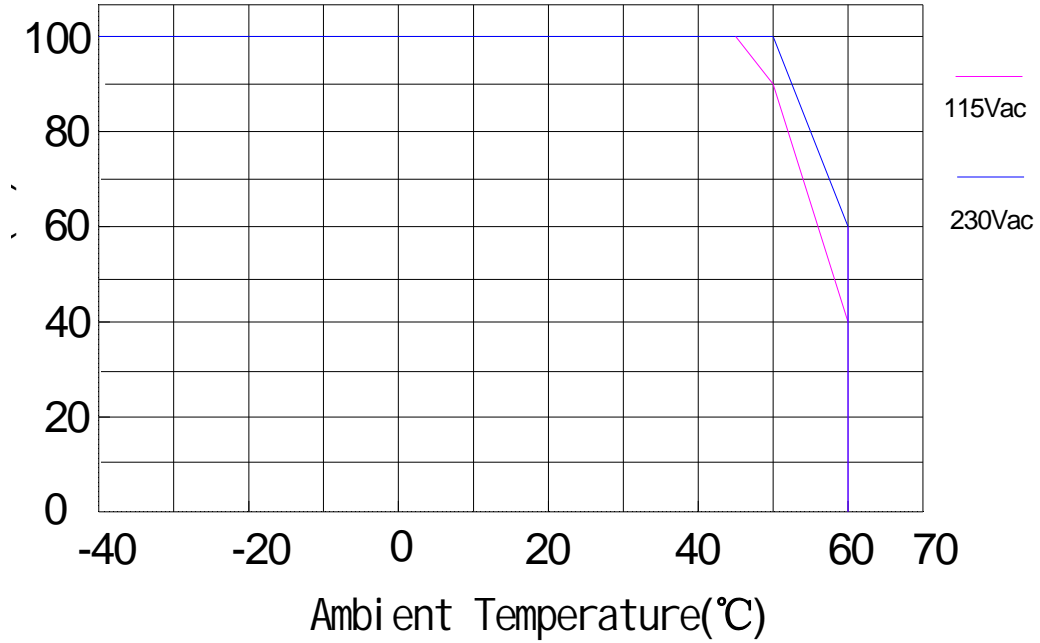
Temperature vs. Load curve
