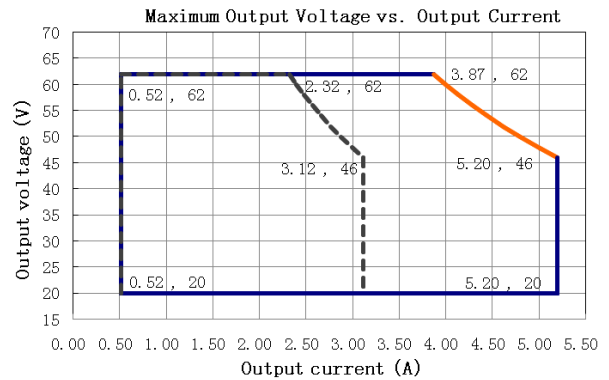
LCP-240X368Z
