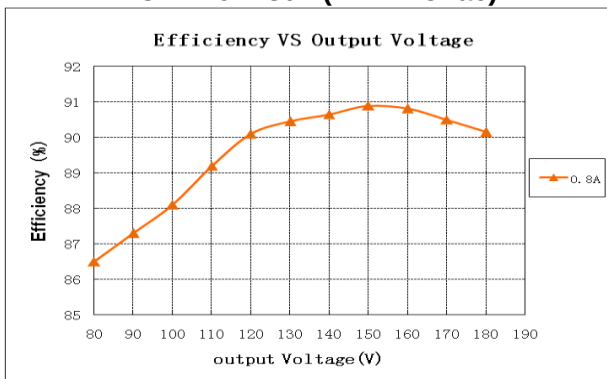
LCP-240X180Z (Vin=115Vac)
