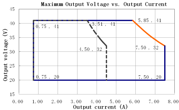
LCP-240X180Z
