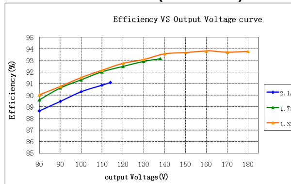
LCP-240X180Z (Vin=230Vac)
