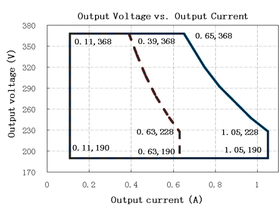
LCP-240X368Z
