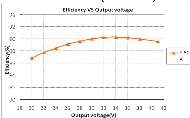
LCP-240X041Z (Vin=115Vac)
