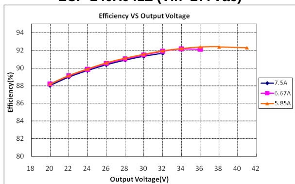
LCP-240X041Z (Vin=277Vac)
