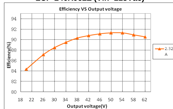
LCP-240X062Z (Vin=115Vac)
