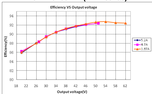
LCP-240X180Z (Vin=115Vac)
