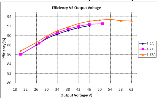
LCP-240X180Z (Vin=230Vac)
