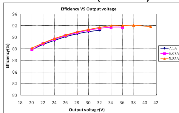
LCP-240X041Z (Vin=230Vac)
