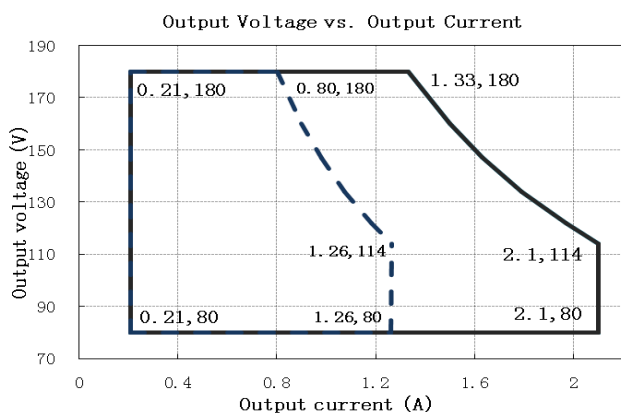
LCP-240X180Z
